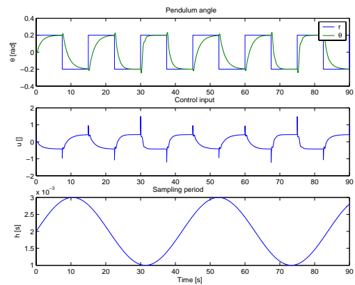
Fig. 7. Motion of the T pendulum under a sinusoidal sampling period
