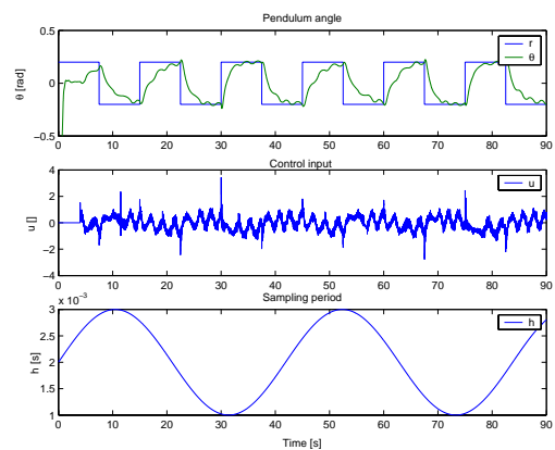
Fig. 9. Experimental motion of the T pendulum under a sinusoidal sampling period
