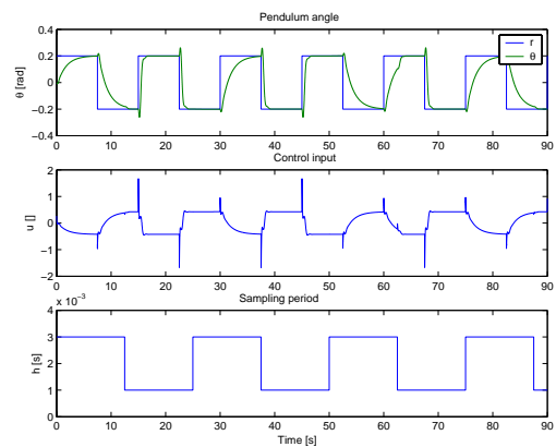
Fig. 8. Motion of the T pendulum under a square sampling period
