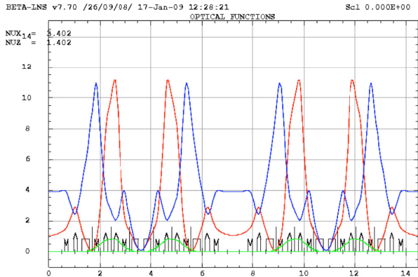
Figure 2: Horizontal (red), and vertical (blue) beta functions.
