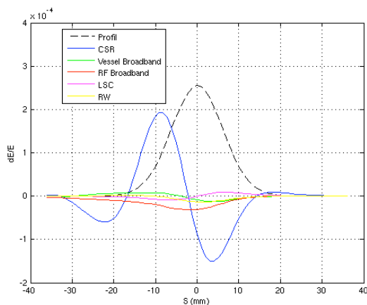
Figure 5: Wakefields distortions along a 1 nC Gaussian bunch at 50 MeV for a bunch length of 20 ps rms.
