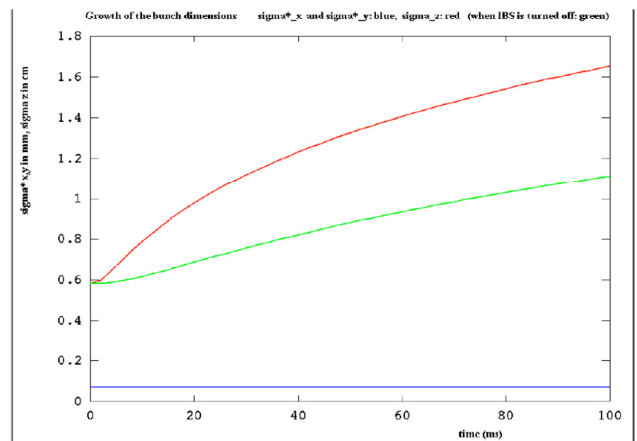
Figure 4: Bunch lengthening by Compton effect only (green) and together with IBS effect (red) versus time.
