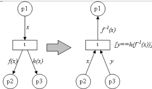
Fig. 5. Parallelism transformation for CPN inversion
