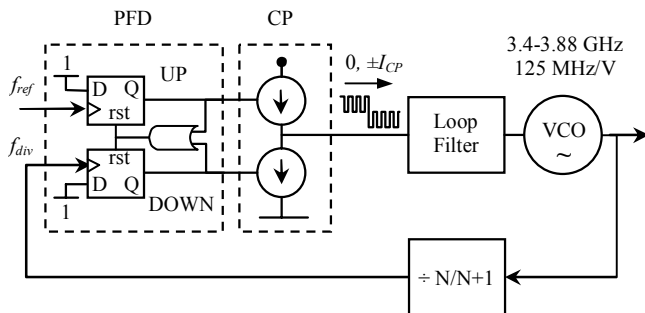
Fig. 1. A model of the fractional- N charge pump synthesizer.
