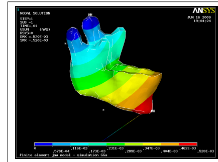
Figure 1. Dynamic jaw simulation for opening in ANSYS with displacement field coloring.
