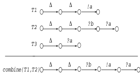
Figure 4. combining initial tours
