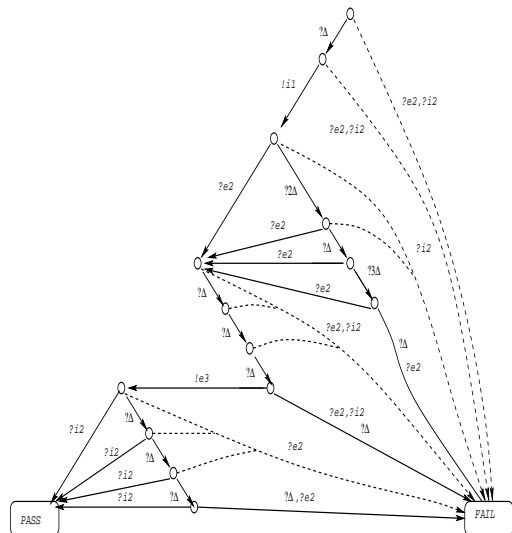
Figure 6. Test case generated for the untimed graph of C_2
