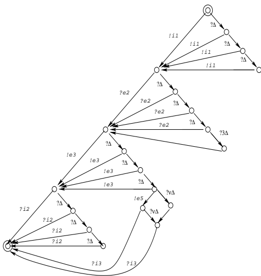
Figure 5. Untimed graph of C_2
