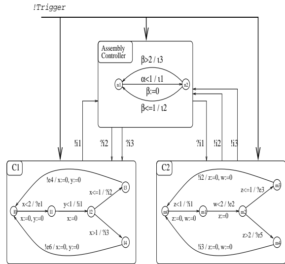
Figure 1. Example of CBRTS
