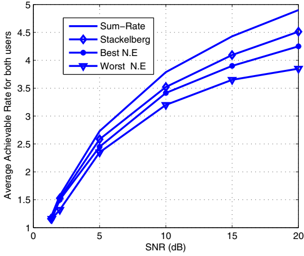
Fig. 6. Average achievable rate for both users versus the signal-to-noise ratio for the centralized and Stackelberg approach. Moreover, the best and worst Nash equilibria for the non-cooperative game are illustrated.
