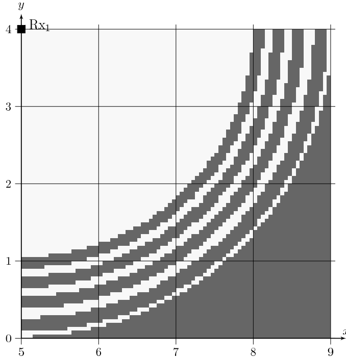
Fig. 7. I_{(1,3)} : showing the influence of the discrete nature of transmit power on connectivity between T_{X_1} and R_{X_1} in the sense of Property 3; (\Delta a, \Delta b) = (0.0625 \text{ m}, 0.0625 \text{ m}) .
