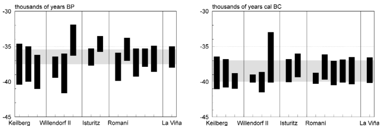
Figure 5 - 14 C dates on charcoal for the early Aurignacian levels of Keilberg-Kirche, Willendorf II, Isturitz, Romani and La Viña. Left: uncalibrated BP ages. Right : CalPal (Weninger and Jöris 2003) calibrated BC ages.
