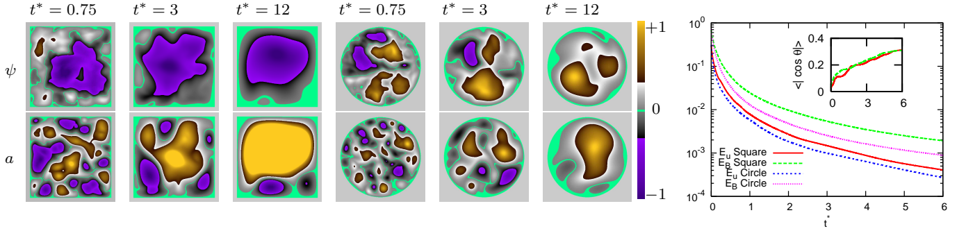
FIG. 1: (Color Online) Visualizations of the stream-function \psi and the vector-potential a for both geometries. Figures for \psi are normalized by the maximum of |\psi| (and \max(|a|) for a ). The values of \max(|\psi|) are from left to right 0.1, 0.05, 0.03; 0.06, 0.03, 0.01; and for \max(|a|) 0.08, 0.06, 0.04; 0.04, 0.03, 0.01. Right: time-evolution of the kinetic and magnetic energy in both geometries. In the inset, the evolution of the absolute value of the relative cross-helicity \langle |\cos(\theta)| \rangle , illustrates the global alignment of the velocity and magnetic field in both geometries. Red solid line: square geometry; green dashed line: circular geometry.
