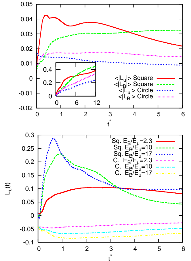
FIG. 2: (Color online) Top: Time evolution of the absolute value of the angular momentum and angular field, averaged over all realizations, normalized by \mathcal{L}_u(0) and \mathcal{L}_B(0) , respectively. In the insert the same quantities are given, normalized by \mathcal{L}_u(t) and \mathcal{L}_B(t) (defined in the text). Bottom: time-dependence of the angular momentum L_u in the square and circular geometry, normalized by \mathcal{L}_u(0) . The influence of the magnetic pressure on the spin-up in the square container is illustrated by changing the ratio E_B/E_u , while keeping E_u fixed.
