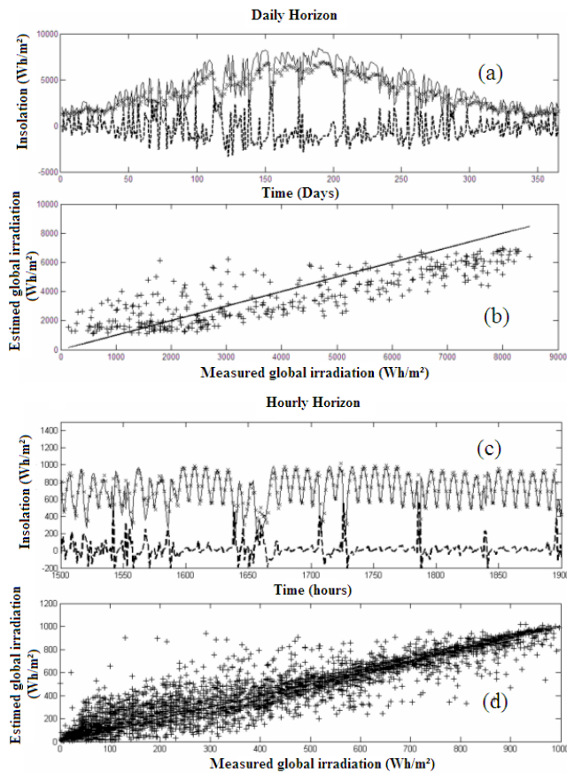
Figure 1: Example of simulated and experimental global solar irradiation in Bastia for the daily horizon (a) and in Corte for the hourly horizon (c). Dashed line is the error, solid line is the measured insolation and marks are the prediction. On the bottom corresponds to the correlation between experimental and simulated global irradiation in Bastia for the daily horizon (b) and in Corte for the hourly horizon (d).
