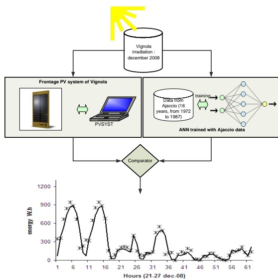
Figure 2: Comparison between computed and measured energy generated with the frontage PV system used in experimentation.
