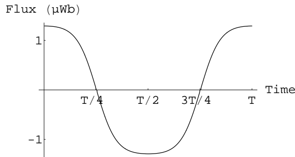
Fig. 4. Cut flux for an excitation of the string Y_I = 10\text{mm} along y . String altitude: d = 5\text{mm} . Magnet position L/4 : neck pickup.
