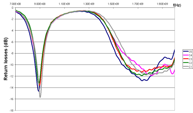
Fig. 5 : Return loss of each element
