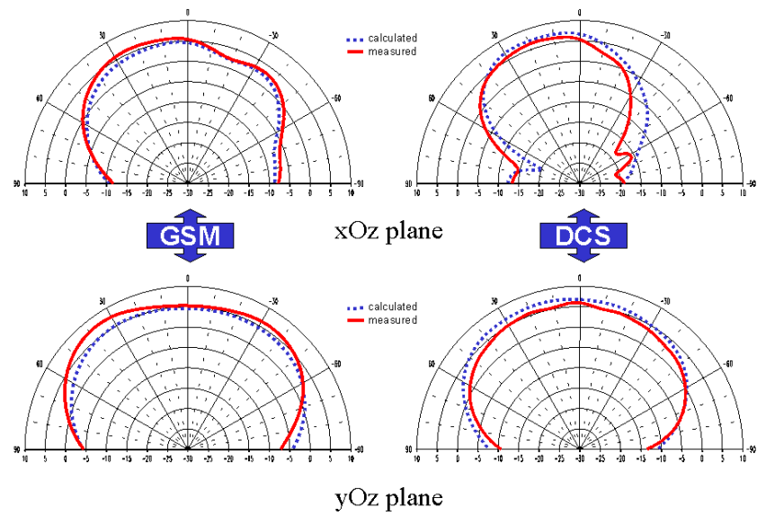
Fig. 6 : Comparative radiation patterns
