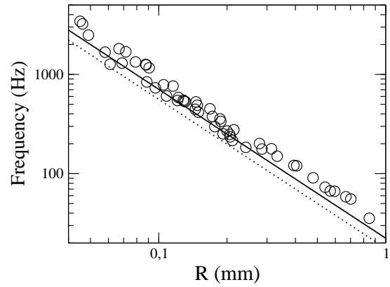
FIG. 6: Eigen frequency as a function of the drop size. The dotted and full lines are calculated using Equ. 6 respectively
