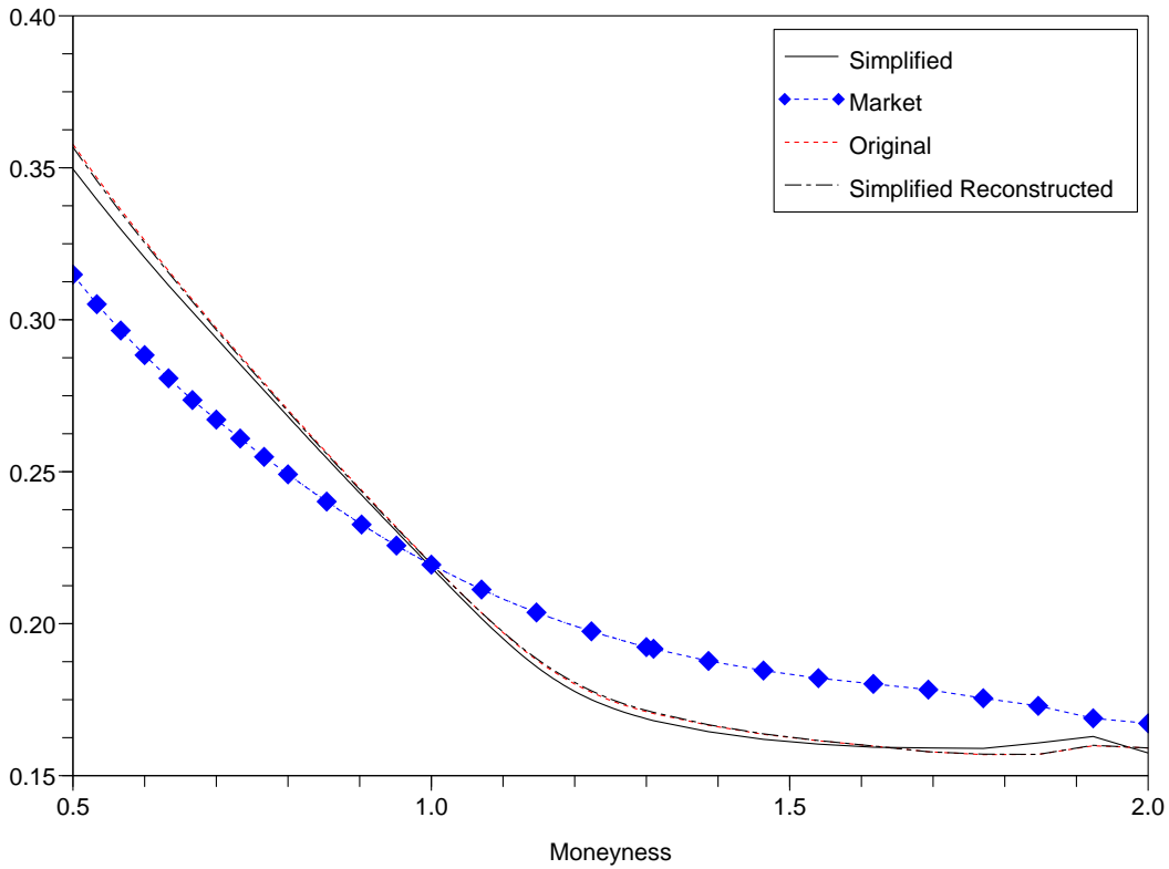
Figure 9: Implied volatility of the index.
