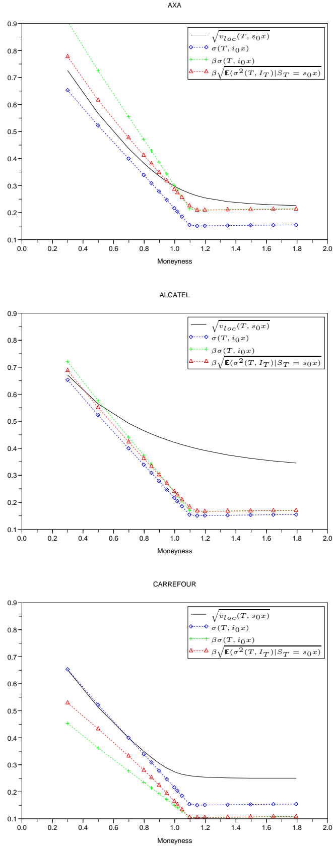
Figure 1: Local volatility x \mapsto \sqrt{v_{loc}(T, s_0 x)} together with x \mapsto \sigma(T, i_0 x) , x \mapsto \beta_{hist} \sigma(T, i_0 x) and x \mapsto \beta_{hist} \sqrt{\mathbb{E}(\sigma^2(T, I_T) | S_T = s_0 x)} when \eta is set to zero for AXA, ALCATEL and CARREFOUR.
