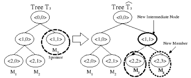
Fig. 2. TGDH - join protocol
