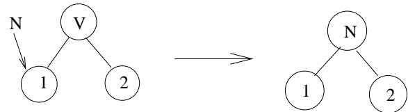
Fig. 6. Adding a node: first case
