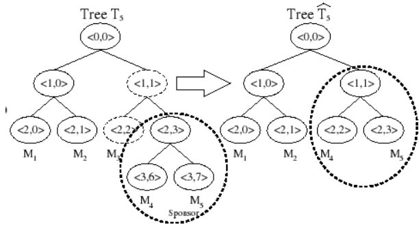
Fig. 3. TGDH - leave protocol
