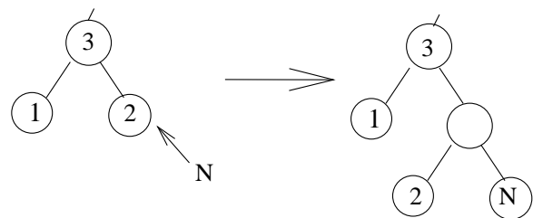
Fig. 7. Adding a node: second case
