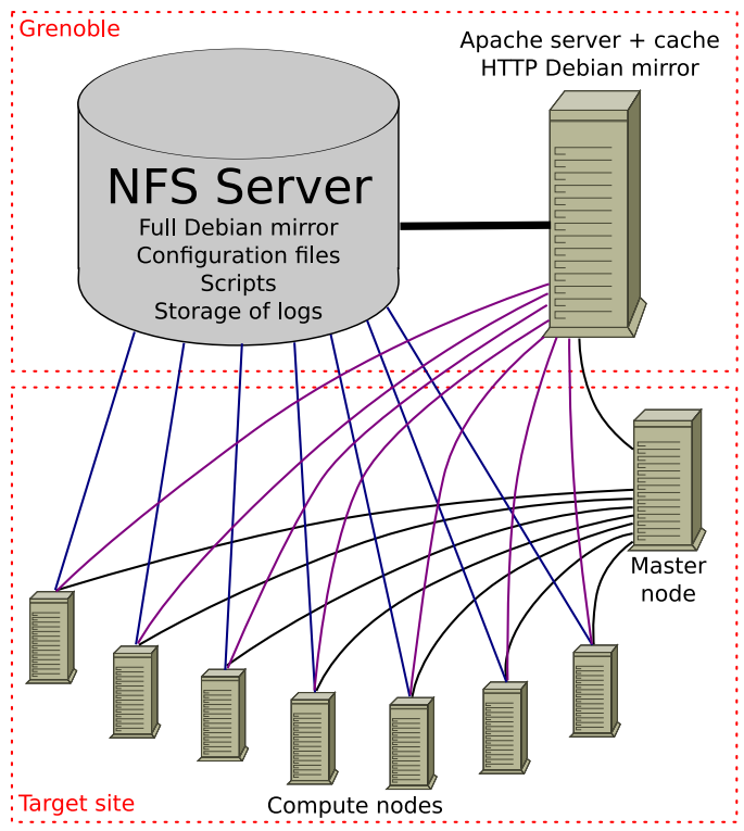
Fig. 4. Software infrastructure
