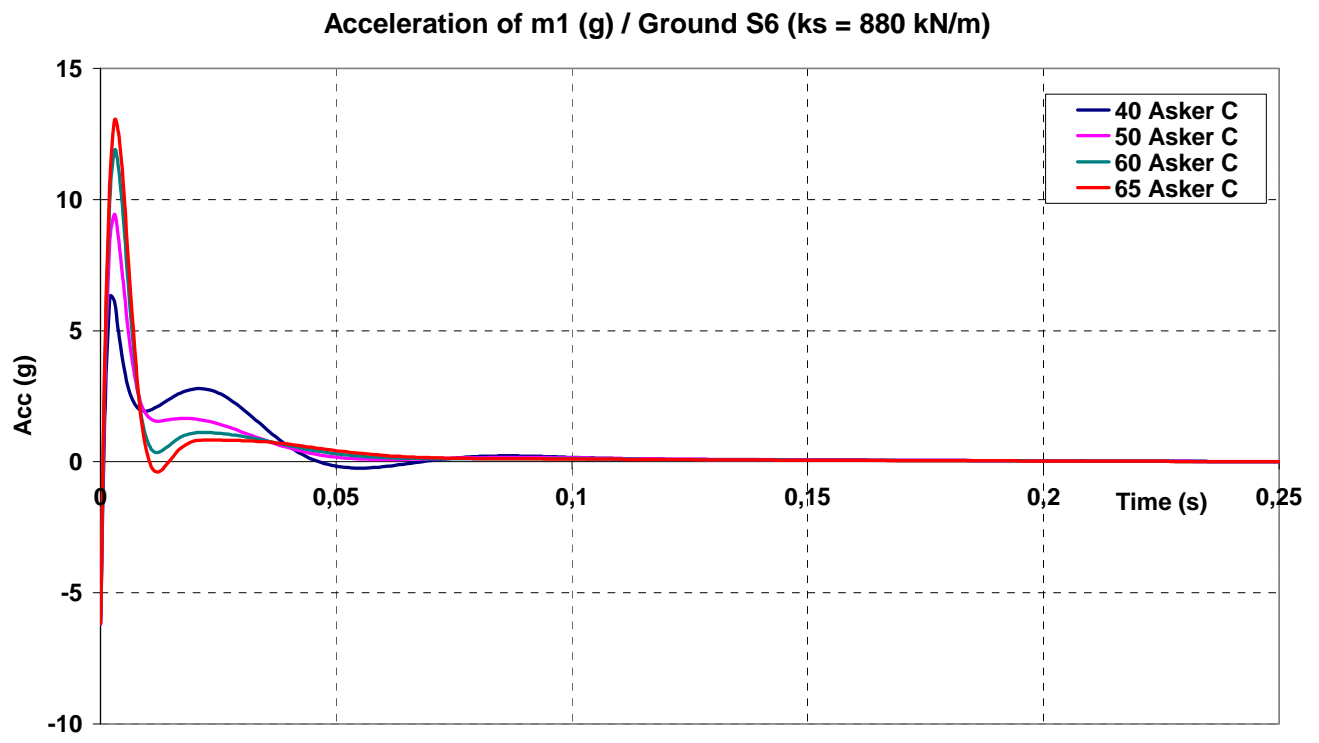
Figure 10 Acceleration of the mass m_1 [g] for soil S6 (ground stiffness k_s = 880 kN/m); load frequency 1.5 Hz.
