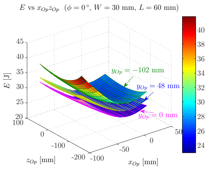
Figure 10: Energy as a function of x_{Op} and z_{Op} for a 30mm×60mm rectangular path
