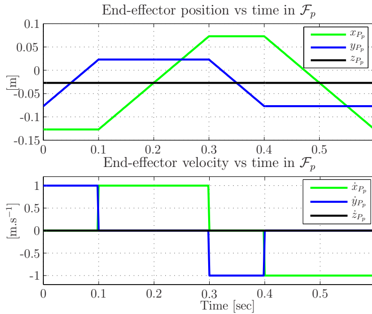
Figure 5: Test trajectory for a rectangular path of size 0.05\text{m} \times 0.10\text{m}
