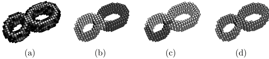
Fig. 8. Experiments on 3D artificial images. The convergence threshold on the number of tunnels b_1 is given for each image. (a) voxels of a 2-torus object. Each voxel belongs to a different region. (b) 2-torus with b_1 \rightarrow 0 . The object is divided into three main regions, none of them having any tunnel. (c) 2-torus with b_1 \rightarrow 1 . One of the two main regions has a tunnel and the other one has none. Two 1-torus are not obtained due to the order in region merging. (d) 2-torus with b_1 \rightarrow 5 . Actually, b_1 increases until reaching its maximal value (2) driven by voxels data.
