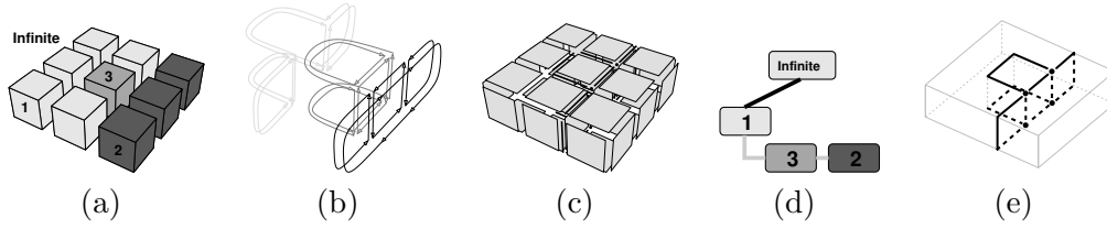
Fig. 2. The different parts of the topological map used to represent an image. (a) 3D image. (b) Minimal combinatorial map. (c) Intervoxel matrix (embedding). (d) Inclusion tree of regions. (e) Cellular representation of the same topological map.
