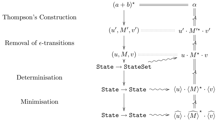
Figure 4: Proof and code relationship.
