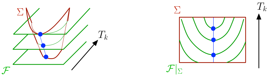
Figure 11: Tangency changes the leaf: we can not conclude
