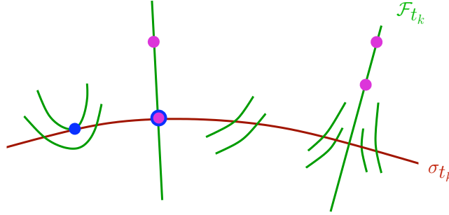
Figure 7: Different possibilities of tangency respectively transversality
