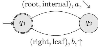
Figure 2: A deterministic tree walking automaton.
