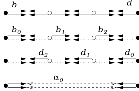
Fig. 4. A 2-G-map G (top row) from which the two white vertices are to be removed, yielding a map G' (bottom row). The connecting walks CW_{G,G'}^0(b) = (b = b_0, b_1, b_2) (second row) and CW_{G,G'}^0(d) = (d = d_0, d_1, d_2) (third row).
