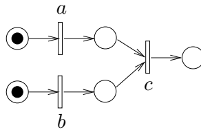
Figure 3: An occurrence net.
