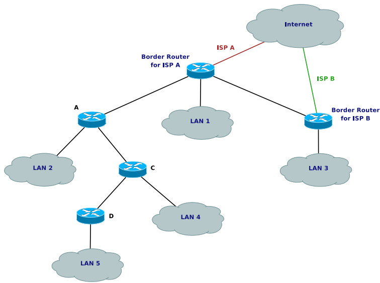
Figure 2.14: Multihomed Site with 2 Border Routers
