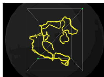
Fig. 4. DNA's 3D model based on biophysical data
