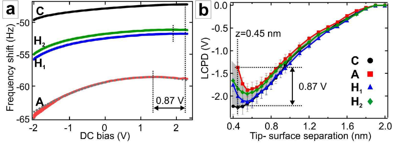
FIG. 3: (Color online) a- Spectroscopic curves computed above the four sites at z = 0.45 nm. A shift of 0.87 V is noticed between anionic (A) and cationic (C) sites. b- Distance dependence of the LCPD above the four sites derived from the spectroscopic curves. In the short-range regime, the LCPD exhibits a resonance-like and site-dependent behavior.
