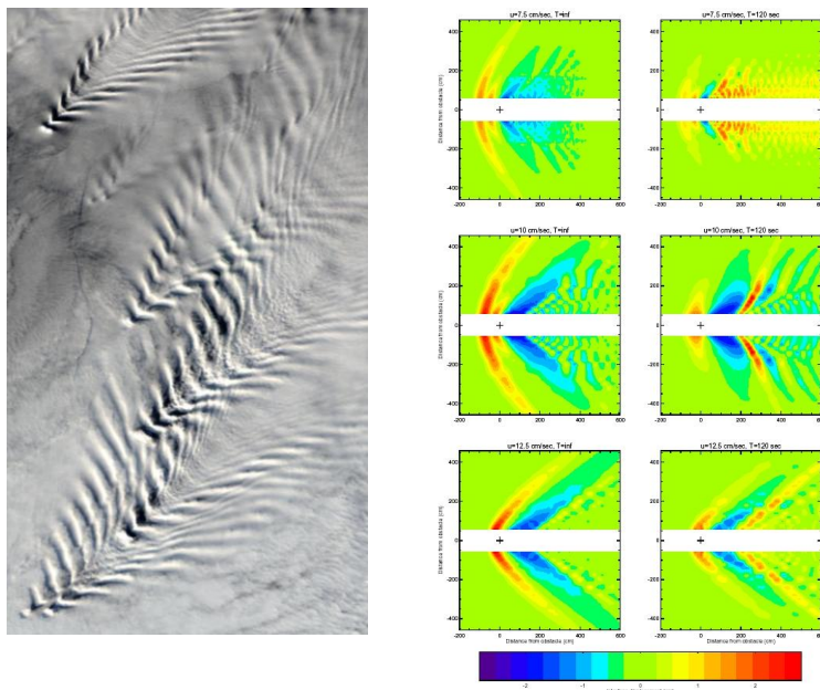
Figure 1. Internal gravity waves produced behind islands in the atmosphere (left) and in a laboratory model (right), from [5]. The color maps indicate fields of vertical displacement for the interface without Coriolis force (first column of three views), and with Coriolis force (second column). The three rows correspond respectively to a flow velocity lower, equal and higher than the wave propagation velocity. The main effect of rotation is to reduce the lateral extension, in particular for the bow wave, but it does not introduce asymmetry between the two sides in this regime (the total width of the domain is 8 m).
