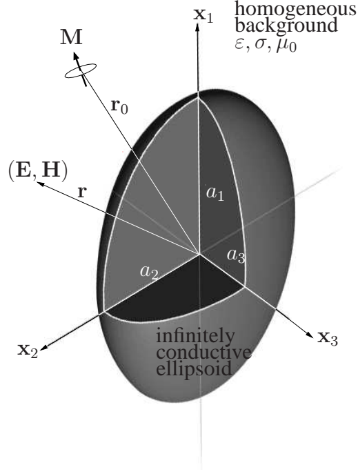
FIG. 1. Problem geometry
