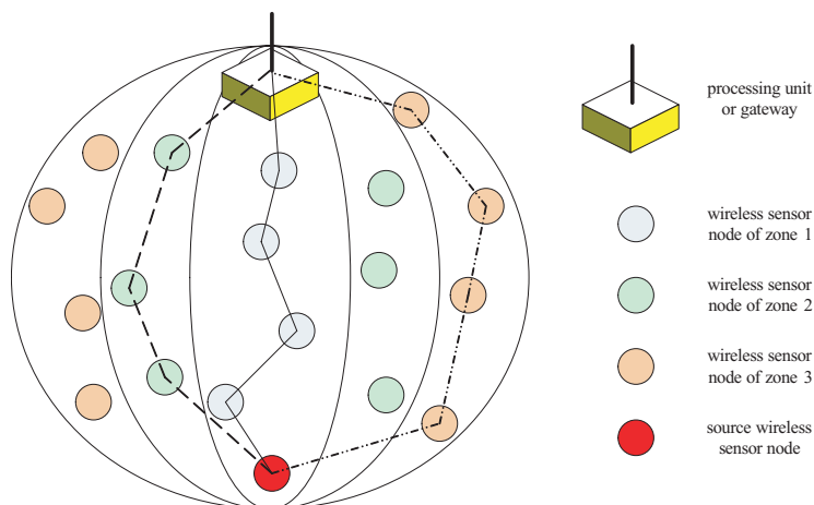
Fig. 3 Value zones as seen from the source node towards the sink, where the value of each zone obeys Zipf's Law.
