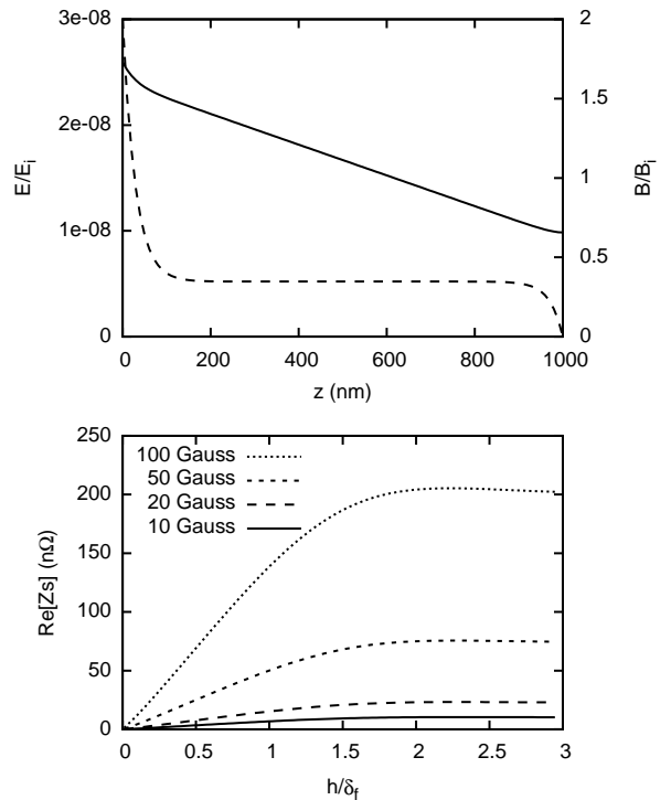
Fig. 3: (a) Electric (solid line) and magnetic (dashed line) field amplitudes in the superconducting slab of thickness h = 1 \mu\text{m} . The superconductor characteristic parameters \delta_f , \lambda_V and l correspond to the niobium layer used in our experiment (see section “Numerical results”). The bias field applied perpendicularly to the slab is B = 100 \text{ G} . The fields are expressed in units of the incident electromagnetic field amplitude. (b) Real part of the surface impedance as a function of h (in units of \delta_f ) for different external bias field B
