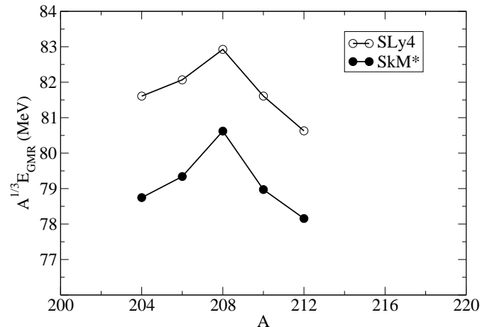
FIG. 1: Excitations energies of the GMR (times A^{1/3} ) in ^{204-212}\text{Pb} isotopes calculated with constrained HFB method and the SLy4 and SkM* interactions
