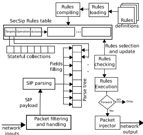
Fig. 4. SIP message traversal through SecSip runtime.
