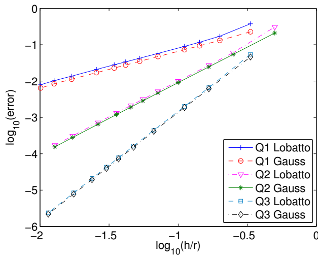
FIG. 11. Error in H^1 norm, by using Gauss or Gauss-Lobatto rules for the 2-D case. The model case is a square meshed in triangles split in quadrilaterals.
