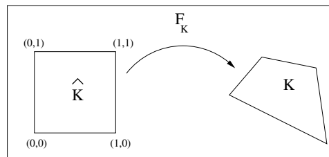
FIG. 2. F_K for two dimensions.
