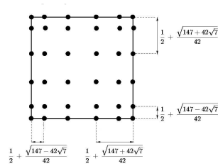
FIG. 3. 2D Gauss-Lobatto points for r = 5 .
