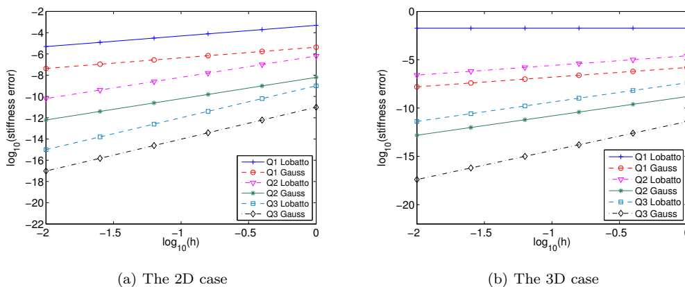
FIG. 7. Curves of convergence for a non uniform mesh, concerning the error of quadrature on the stiffness matrix by using Gauss-Lobatto or Gauss rules.
