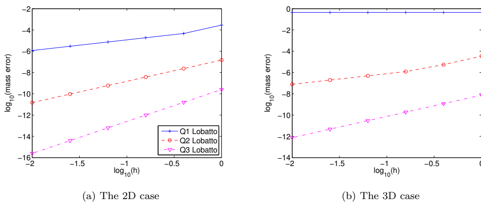
FIG. 6. Convergence curves for the mass matrix using Gauss-Lobatto: non uniform meshes.
