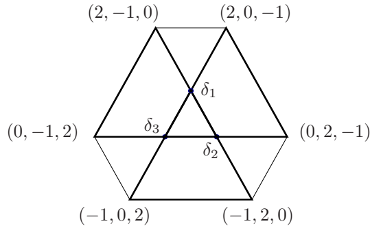
Figure 2: trace of \Sigma (convex hull) and of \{\eta - \delta_k, \eta \geq 0, |\eta| \geq 2, k \in \{1, 2, 3\}\} (union of three triangles) on the hyperplane \{x_1 + x_2 + x_3 = 1\} of \mathbb{R}^3
