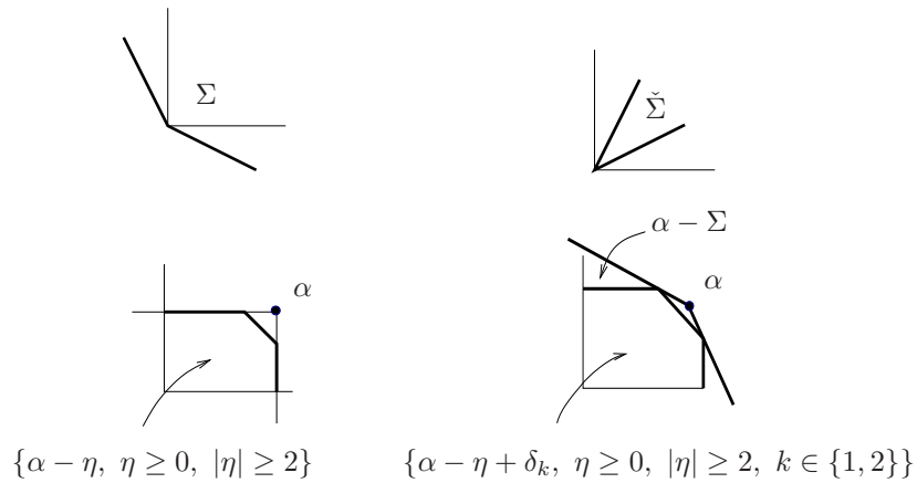
Figure 1: cone \Sigma and related sets in dimension 2
