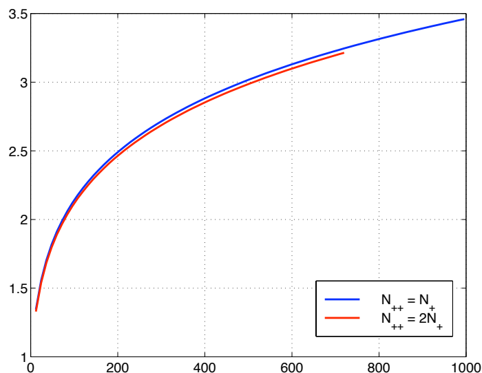
Figure 7: Evaluation of the H^{1/2}(\Lambda) operator-norm of \pi_N
