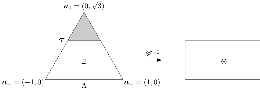
Figure 2: The homographic transformation from \mathcal{Z} onto \Theta
