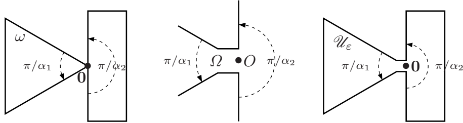
FIGURE 4. Example of domains \omega , \Omega and \mathcal{U}_\varepsilon in the multiply connected case ( \alpha_1 = 3 , \alpha_2 = 1 ).
