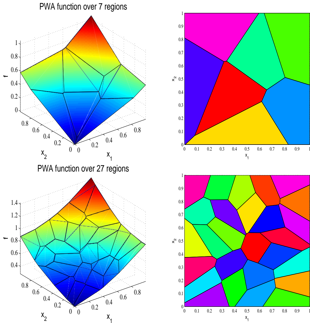
FIGURE 1. Mapping the uniform to a discrete discrete distribution in dimension d = 2 . Upper row: seven atom points, lower row: twenty-seven atom points. Left column: the potential V(u) = w^*(u) . Right column: the corresponding partition of the space \mathcal{U} .
