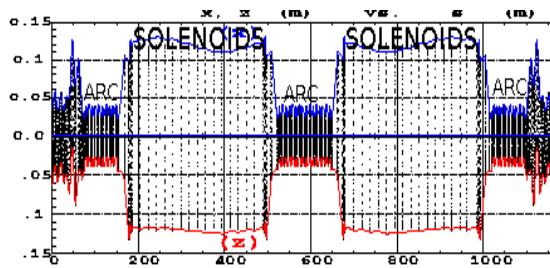
Fig. 2 : Beam tracks (from ray-tracing) and envelopes (from matrix transport) in defect free ring (blue : horizontal, red : vertical).
