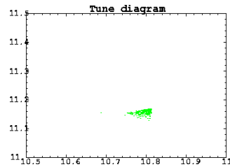
Fig. 3 : Footprint in tune diagram, chromaticity corrected, given a beam with \epsilon_{x,z} = 6 \pi cm norm., \delta p/p = \pm 4\% .
