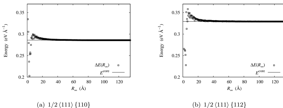
Figure 3. Variation with the cylinder radius R_\infty of the energy difference \Delta E(R_\infty) = E(R_\infty) - \frac{1}{2}b_i K_{ij}^0 b_j \ln(R_\infty/r_c) showing the convergence to E^{\text{core}} for 1/2 \langle 111 \rangle \{110\} and 1/2 \langle 111 \rangle \{112\} edge dislocations in \alpha -iron ( r_c = b \simeq 2.473 \text{ \AA} ).
