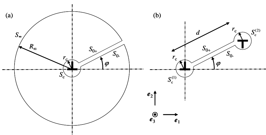
Figure 1. Definition of the contour used to calculate the dislocation elastic energy. (a) Isolated dislocation. (b) Isolated dislocation dipole.
