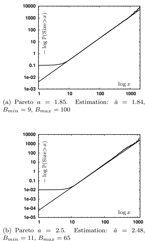
FIGURE 3. Synthetic traces with 10^6 flows with a Pareto distribution
