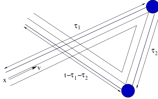
FIGURE 4. The tube T(t, c_1, c_2) corresponding with the third term in the series expansion giving the particle density
