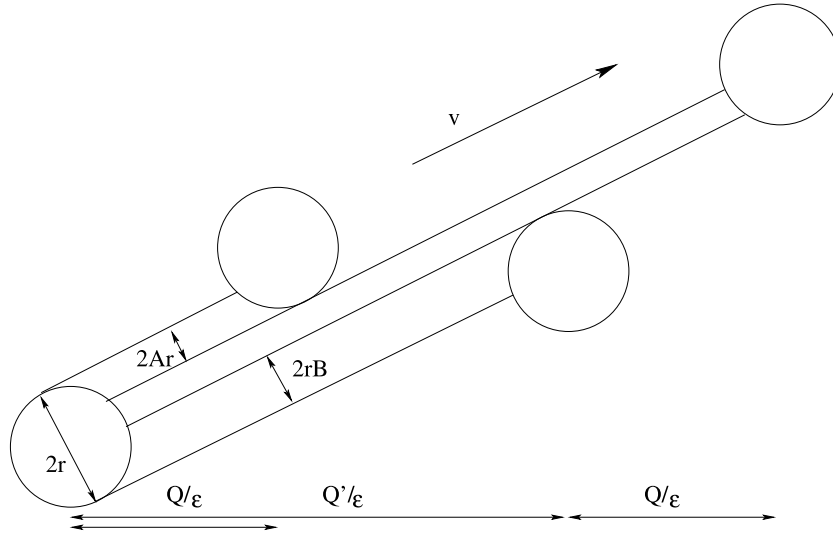
FIGURE 19. Collision pattern seen from the surface of one obstacle. Here, \epsilon = 2r/v_1 .
