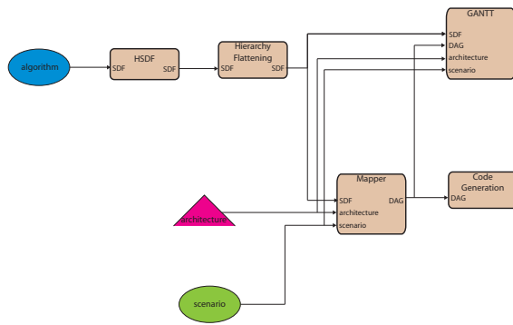
Fig. 9. PREESM Workflow
