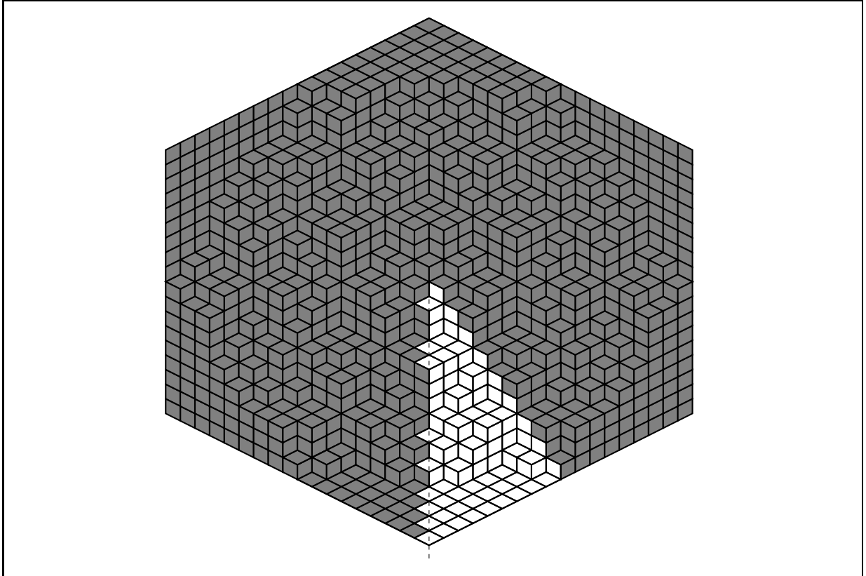
Figure 23: A TSSCPP, is a plane partition with all symmetries of the hexagon+ self complementarity (i.e. imagine that it is a pile of cubes within a big cube, then it must be equal to its complement). A TSSCPP configuration is completely determined by a partition of 1/12 th of the hexagon (the white region).
