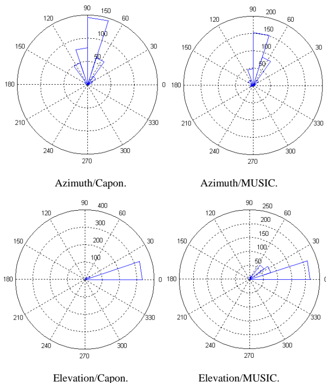
Fig. 13: Azimuth and elevation angle estimations in Paris (field test 1), for the first path.
