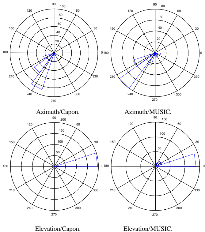
Fig. 10: Azimuth and elevation angle estimations in motorway area.
