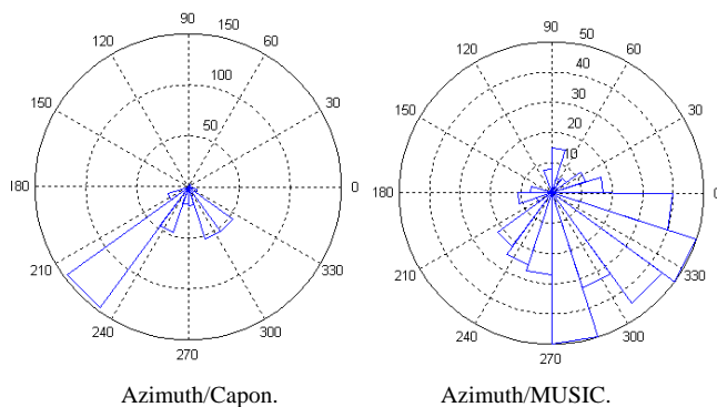
Fig. 14: Azimuth angle estimations in Paris (field test 1), for the second path.
