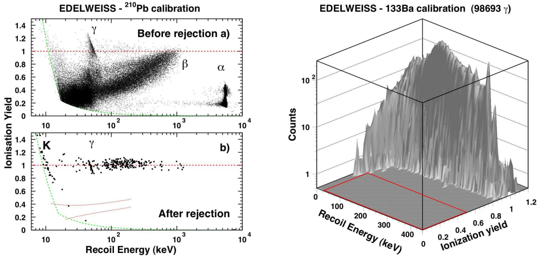
Figure 1: Ionization yield as a function of recoil energy recorded in EDELWEISS InterDigit detectors (ID) recorded in calibrations with a ^{210}\text{Pb} (left) and ^{133}\text{Ba} (right) source (taken from Ref. 20 ). The panels (a) and (b) show the effect of surface event rejection on the population of \gamma , \beta and \alpha rays from the source (see text for explanation). The remaining \gamma and K-shell X-ray population along the ionization yield of one in panel (b) comes from natural background. The right panel show the rejection for \gamma -rays.
