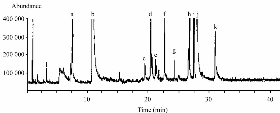
Figure 2. Chromatogram obtained by GC/MS analysis for a NAPP - \text{NH}_2\text{Cl} mixture;
