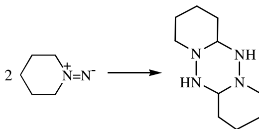
Dipyridododecahydro-s-tetrazine ( m/z = 196 )
