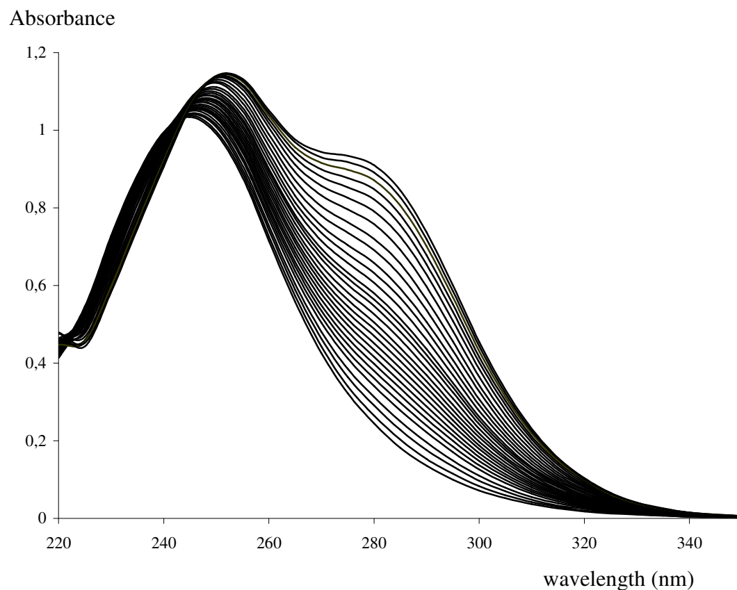
Figure 3. UV absorption spectra of NAPP – \text{NH}_2\text{Cl} mixture at \text{pH} = 11.5 ;
