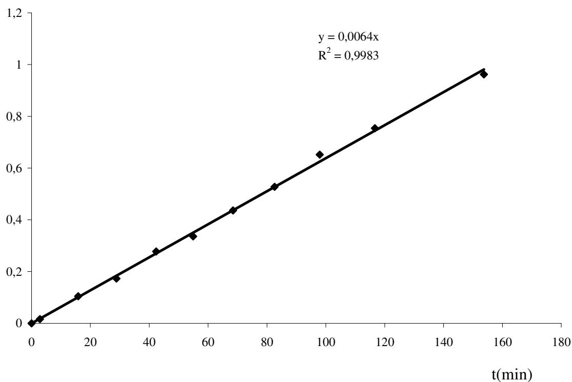
Figure 5. Determination of the kinetic parameters in the oxidation of N -aminopiperidine with chloramine (first step of the reaction monitored by HPLC; [\text{C}_5\text{H}_{10}\text{NNH}_2]_0 = 10 \times 10^{-3} \text{ M} , [\text{NH}_2\text{Cl}]_0 = 4 \times 10^{-3} \text{ M} , \text{pH} = 12.89 , T = 25^\circ\text{C} ).
