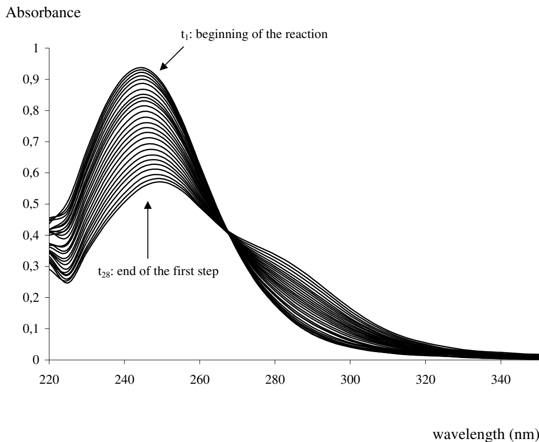
Figure 1. UV absorption spectra of the oxidation of N -aminopiperidine with chloramine (first step; [C_5H_{10}NNH_2]_0 = 20 \times 10^{-3} M , [NH_2Cl]_0 = 2 \times 10^{-3} M , pH = 12.89 , T = 25^\circ C ).
