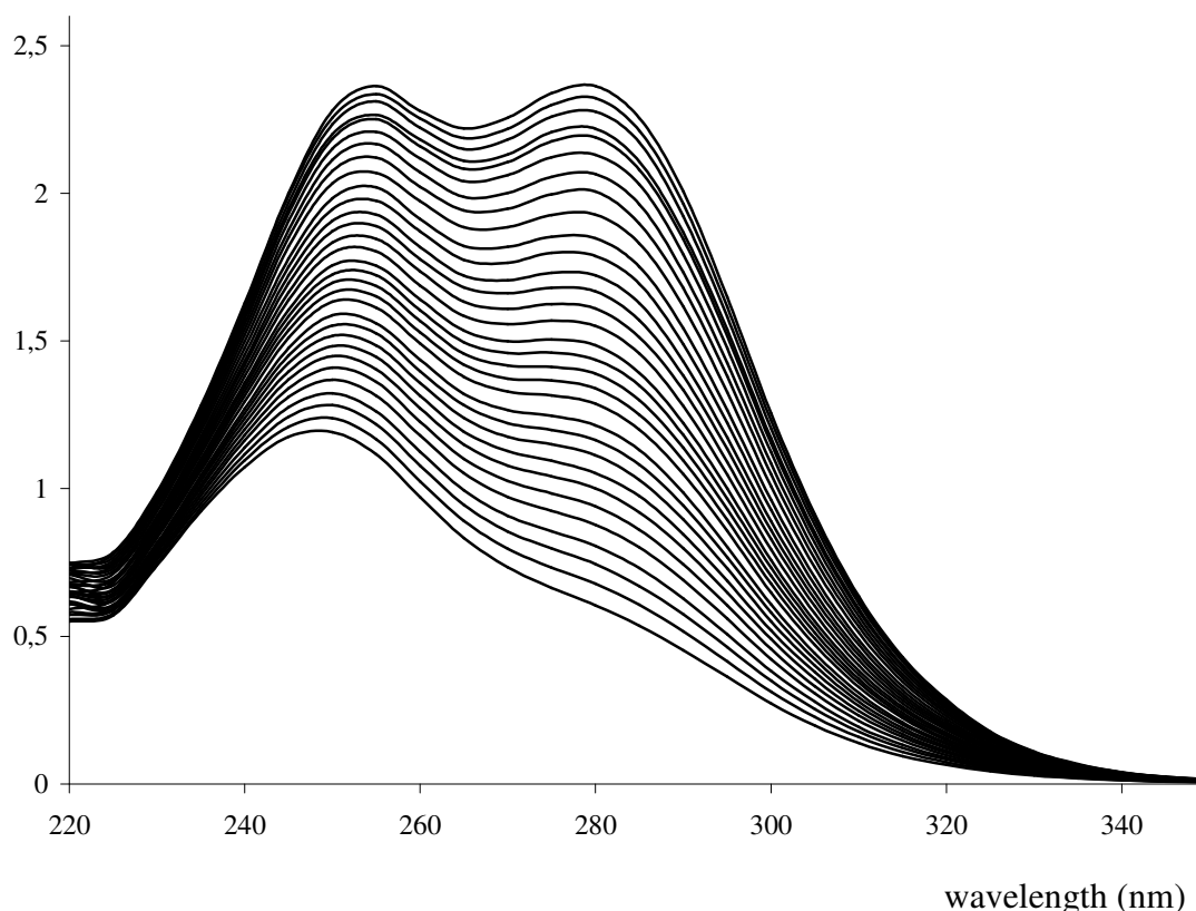
Figure 4. UV absorption spectra of NAPP – NH 2 Cl mixture at pH = 11; ([C 5 H 10 NNH 2 ] 0 = 20 × 10 -3 M, [NH 2 Cl] 0 = 2 × 10 -3 M, T = 25 °C).
