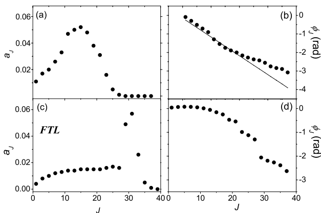
FIG. 2: (a) amplitude a_J and (b) phase \phi_J vs J of the Fourier components at Raman frequency of \langle \cos^2 \theta \rangle(t) for the optimized pulse shape. (c) and (d) same as (a) and (b) for the FTL pulse. The full curve in panel (b) refers to the criteria of complete rephasing of the rotational wavepacket (see text).
