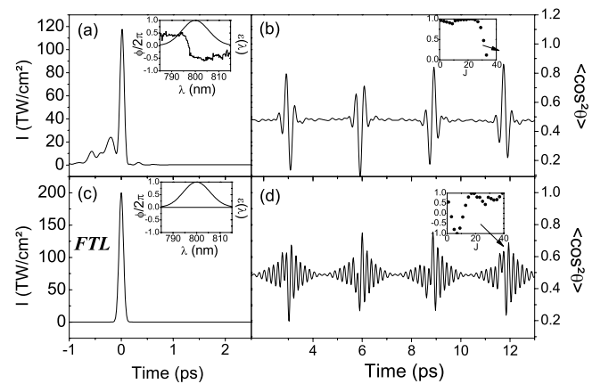
FIG. 1: (a) Optimized pulse shape, (c) FTL pulse with spectral phase and amplitude in insets ; (b) and (d) \langle \cos^2 \theta \rangle(t) induced respectively by these two pulse shapes. The insets in (b) and (d) characterize the rephasing of the wavepacket at t = T_r , i.e. \cos(\omega_J T_r + \phi_J) vs J (see text).
