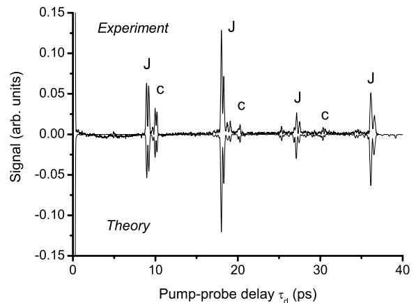
FIG. 5: Probe signal recorded in ethylene at room temperature for a low intensity \mathcal{I}_p = 2 \times 10^{12} \text{ W.cm}^{-2} of the pump laser. J and C -type transients are indicated. The numerical calculation is shown reversed.
