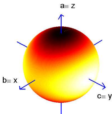
FIG. 1: (Color online) Schematic representation of the potential (6) of a near-prolate molecule on the sphere of coordinates \theta, \chi, r = 1 , where the lowest values of energy are darker. This can be interpreted as the potential in the molecular frame as a function of the polarization axis of spherical coordinates (\theta, \chi) .
