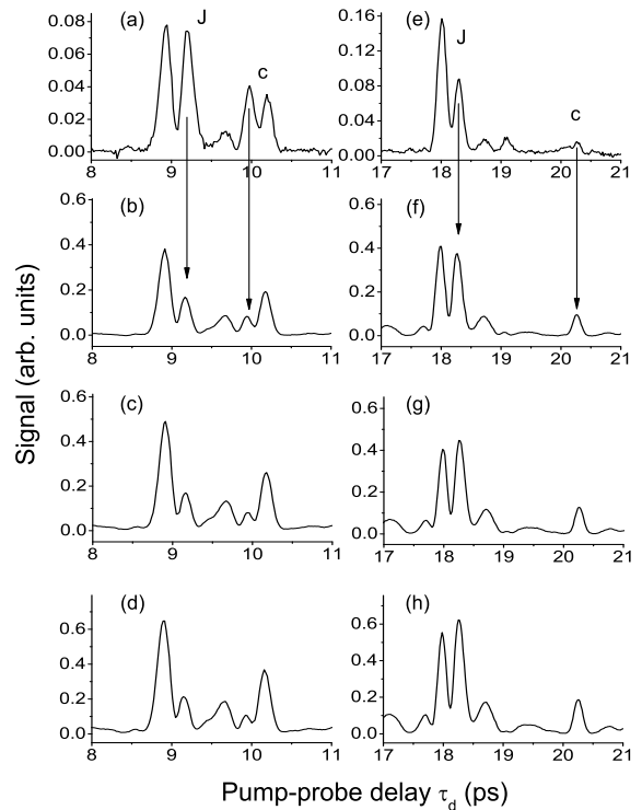
FIG. 6: Probe signals recorded in ethylene exposed to different intensities of the alignment laser: (a, e) 2 \times 10^{12} W.cm -2 , (b, f) 16 \times 10^{12} W.cm -2 , (c, g) 30 \times 10^{12} W.cm -2 , (d, h) 50 \times 10^{12} W.cm -2 . Only the temporal windows that correspond to the first (a-d) and second (e-h) rotational revivals of Fig. 5 are shown.
