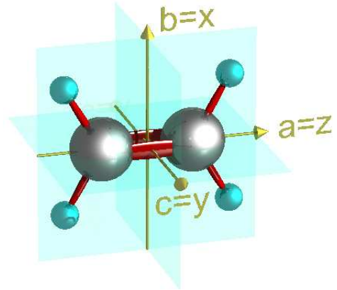
FIG. 2: (Color online) Ethylene molecule depicted with the molecular fixed frame axis x, y, z .
